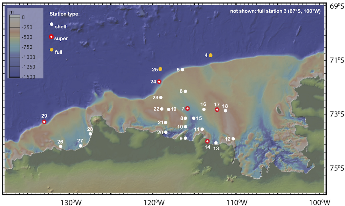
Figure 1. Track and station locations for GEOTRACES Section GP17-ANT.
